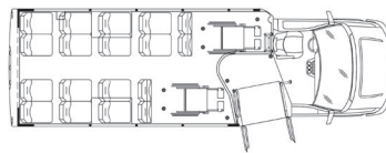
26', 14+4 Passenger, 2 w/c
