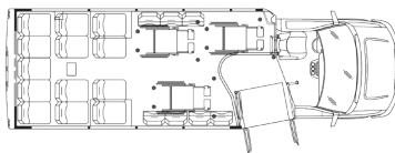
26', 13+7 Passenger, 3 w/c
