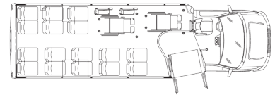
28', 16+4 Passenger, 2 w/c
