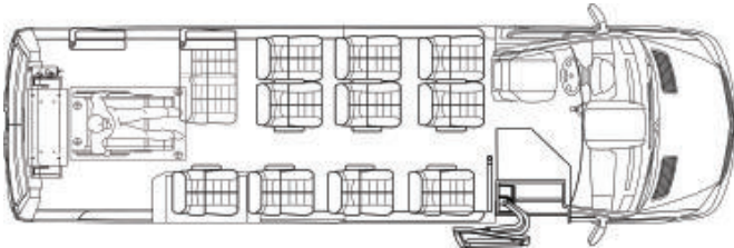
PDPT15 Paratransit Commuter Shuttle (14+1)
