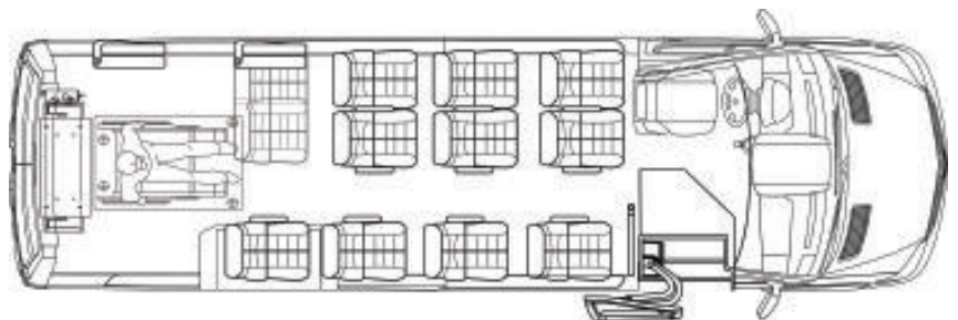
PDPT15 Paratransit Commuter Shuttle (14+1)
